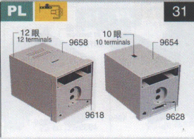
9658:96 × 96 × 120mm 9654:96 × 96 × 120mm
