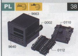
9663:96 × 96 × 100mm
