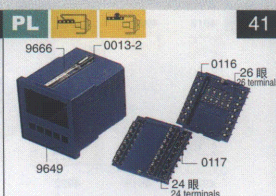
9666:96 × 96 × 120mm
