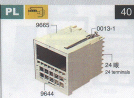
9665:96 × 96 × 100mm
