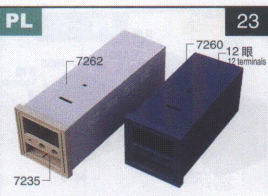
7260:72 × 72 × 150mm 7262:72 × 72 × 200mm
