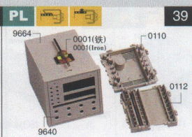
9664:96 × 96 × 120mm
