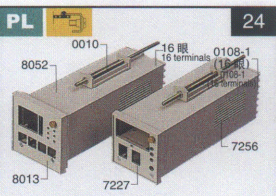
7256:72 × 72 × 200mm 8052:80 × 80 × 200mm
