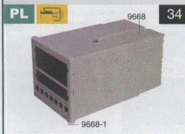
9668:96 × 96 × 178mm
