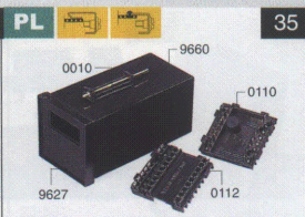
9660:96 × 96 × 180mm
