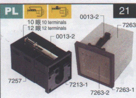
7257:72 × 72 × 110mm 7263:72 × 72 × 80mm
